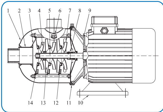
截面图 CHL, CHLK8,12,15,20
